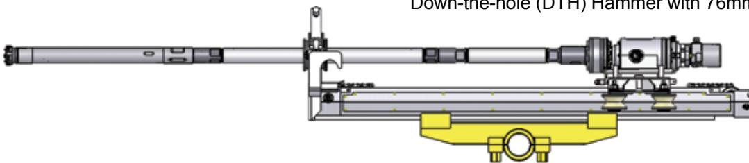
AK 14/80 drilling mast complete with Rotary Head and Down-the-hole (DTH) Hammer with 76mm drill bit
